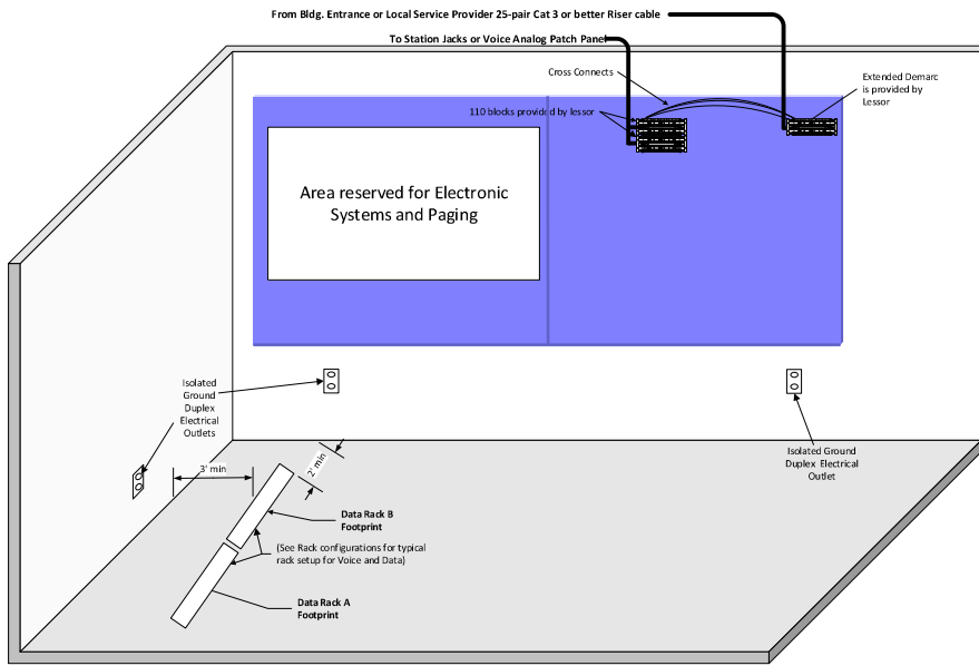
Sample Configuration of Telecommunications Room Layout
